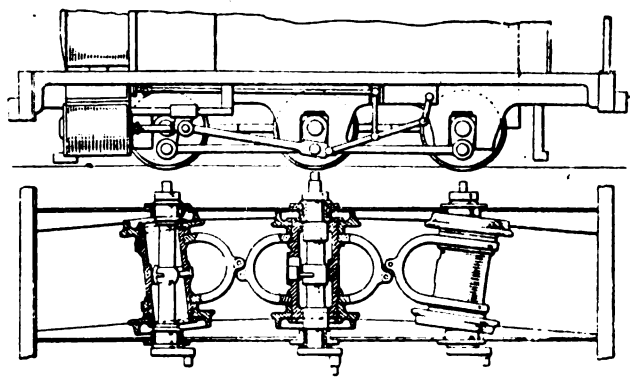
Fig. 4. — Locomotiva Haywood.
